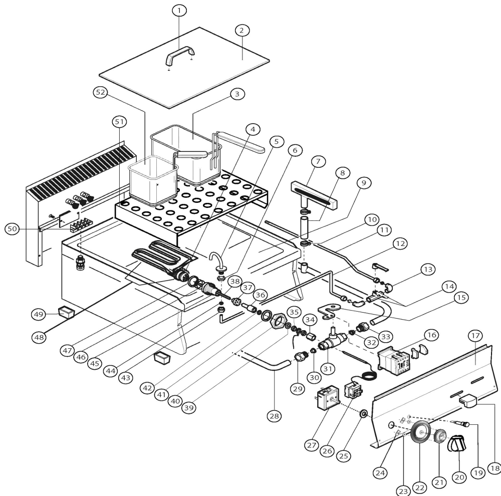
ELECTRIC PASTA COOKER
