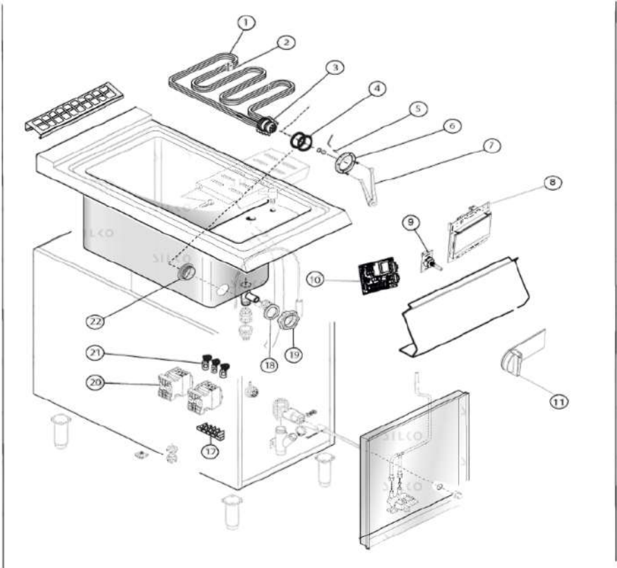
ELECTRIC PASTA COOKER
