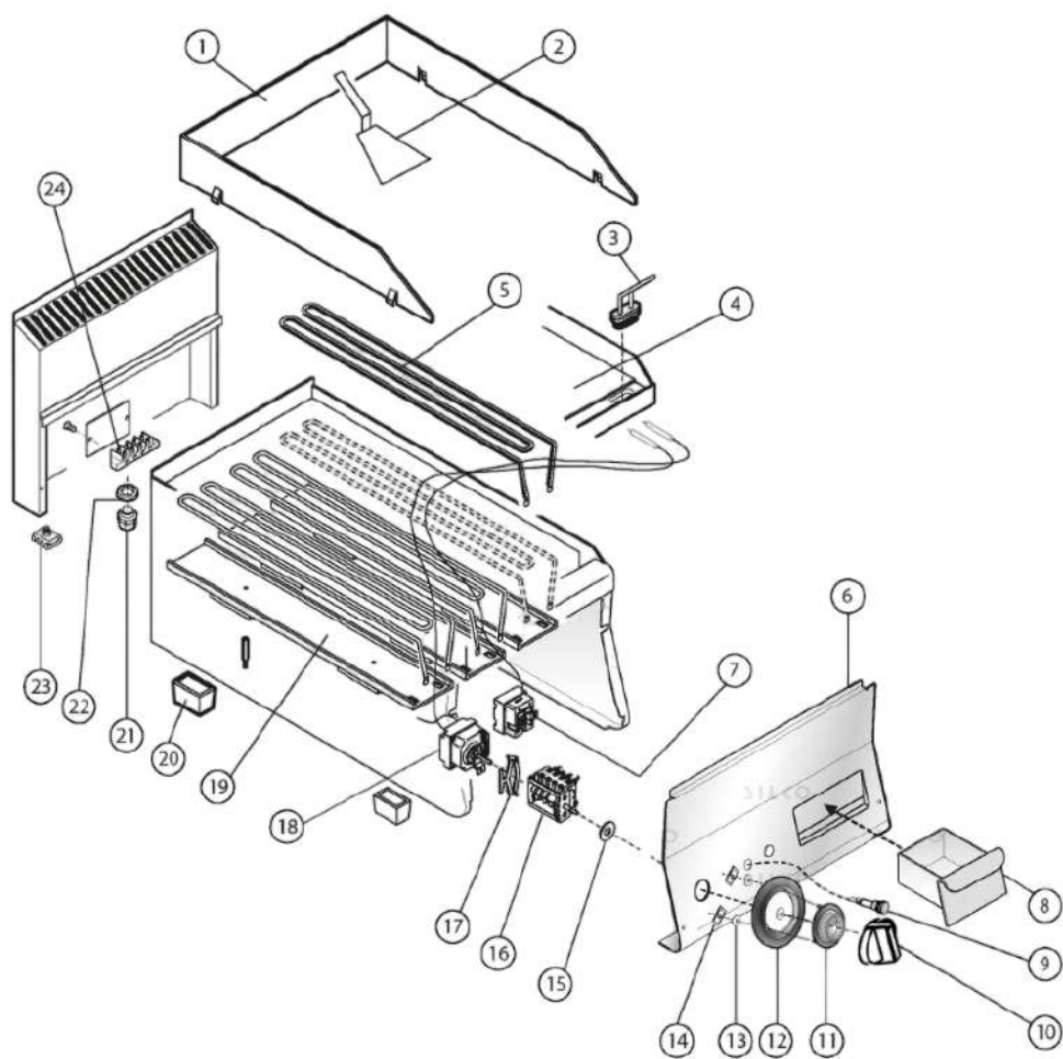
ELECTRIC GRIDDLE
