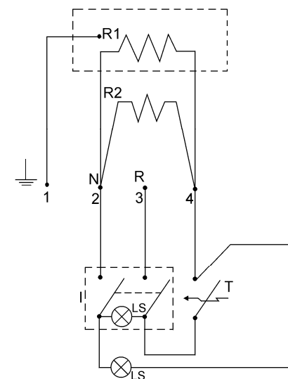
FIG. n°5A - Electrical circuit diagram of the PM PLATE
