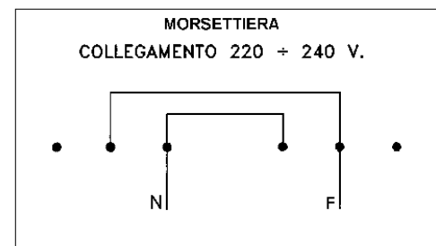
FIG. n°5 - Electrical circuit diagram of the PG PLATE
